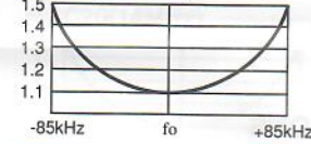
MDC20(14MHz)
